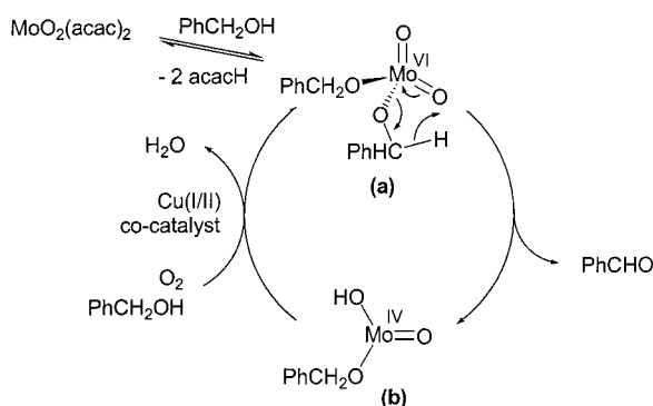
Figure 1. Proposed mechanism for the Mo–Cu–O 2 -catalysed oxidation of PhCH 2 OH; apparently low coordinate species b represented in this figure will have additional neutral ligands, such as alcohol, which have been omitted for simplicity
